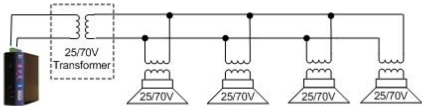
25/70v distribution line using parallel wiring
